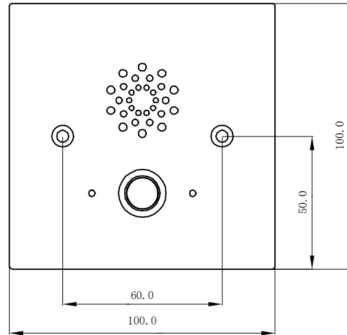
1 FRONT VIEW
